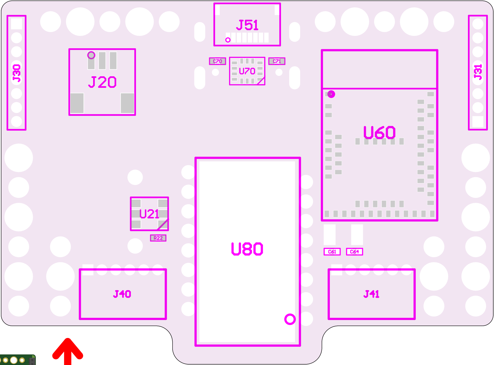
TOP VIEW:
