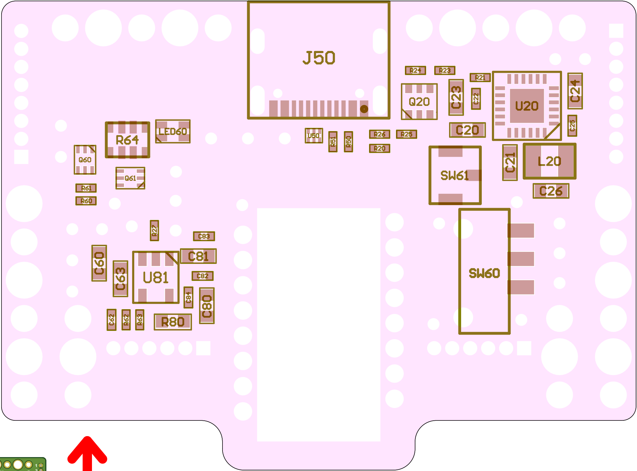
BOTTOM VIEW:
