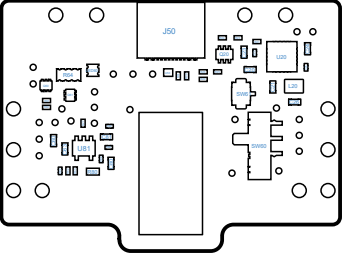
View from Bottom side (Scale 1:1)
