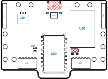
View from Top side (Scale 1:1)
